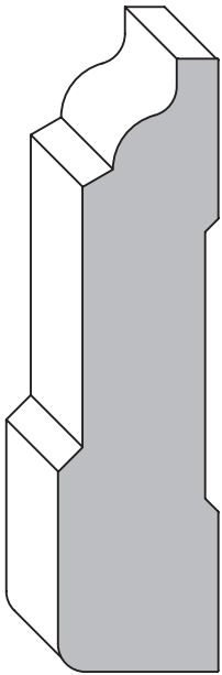
2033 w/ E1E 1/8" 3/4" x (2 7/8" max.)
