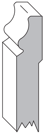
3070 7/16" thick up to 4 1/4" wide
