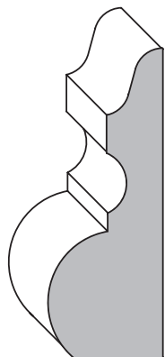
3066 1 1/16" x (1 7/8" max.) Rabbet availability depends on profile
