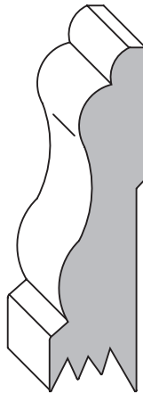
1037 9/16" thick up to 4 1/2" wide
