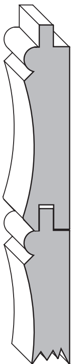
7010 1/2" x 2" (max. face) Add 1/4" for tongue
