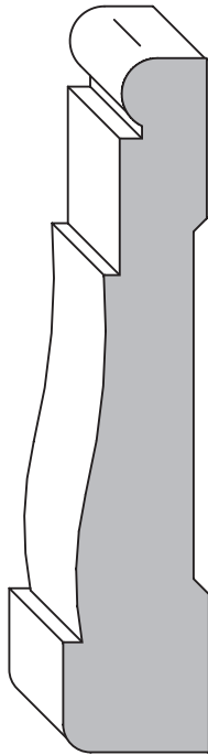
2028 w/ E1E 1/8" 11/16" x (3 3/4" max.)
