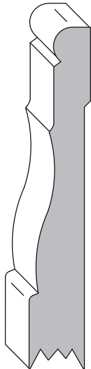
1055 5/8" thick up to 6" wide
