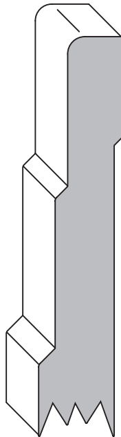
1061 5/8" thick up to 6" wide
