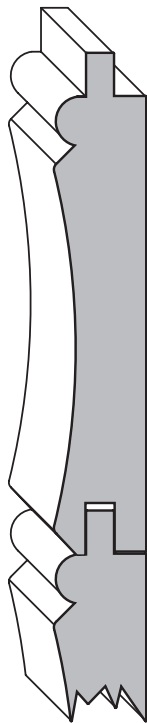
7003 1/2" x 2 1/2" (max. face) Add 1/4" for tongue
