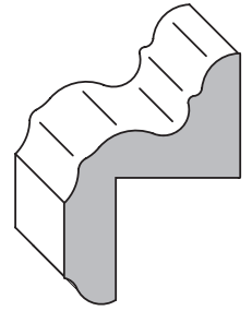
3056 w/ 5/8" rabbet only 5/8" x 1 7/16" (No size alterations)
