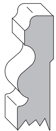
1068 5/8" thick up to 6" wide
