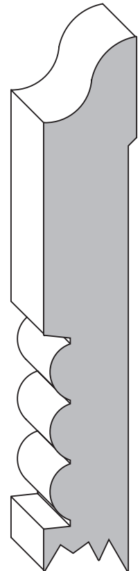
1048 (Beads) 1049 (Nose) 11/16" thick up to 5 3/16" wide
