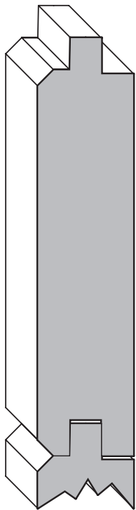
6000 3/4" x 3" (face) Up to 8 3/4" (face) Add 1/4" for tongue
