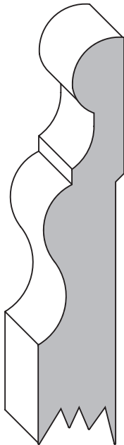
1059 5/8" thick up to 7" wide
