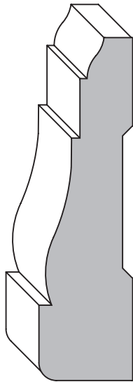
2021 w/ E1E 1/8" 11/16" x (2 1/2" max.)
