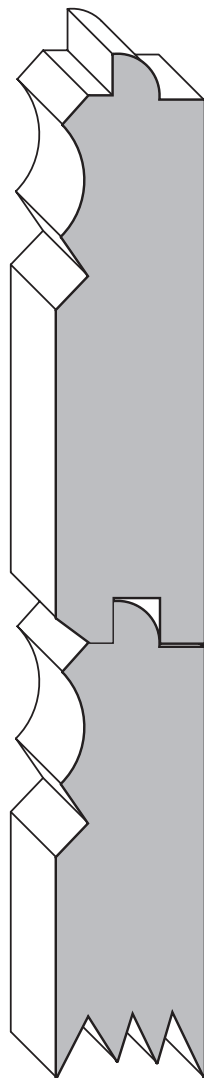
7004 13/16" x 3" (face) 9" (max. face) Add 1/4" for tongue Special setup required
