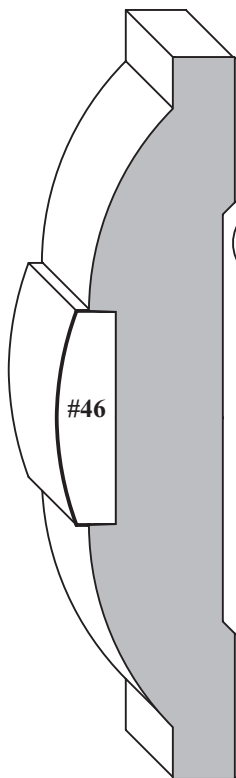
5012 3/4" x (3 3/4" max.) 5/16" x (1 1/8" max.) (Acc. 46 Inlay)
