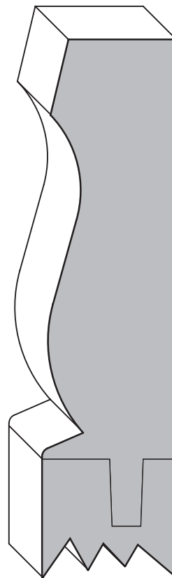
1060 1" x 3 1/8" (Top) Add 1/2" for tongue Bottom can be made up to 9".
