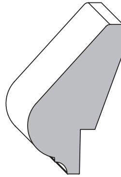
3049 w/ 1/2" rabbet only 3/4" x 1 13/16" (No size alterations)
