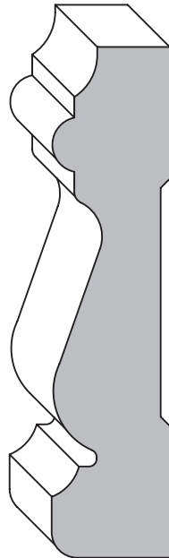
2016 w/ E1E 3/16" 11/16" x (2 15/16" max.)
