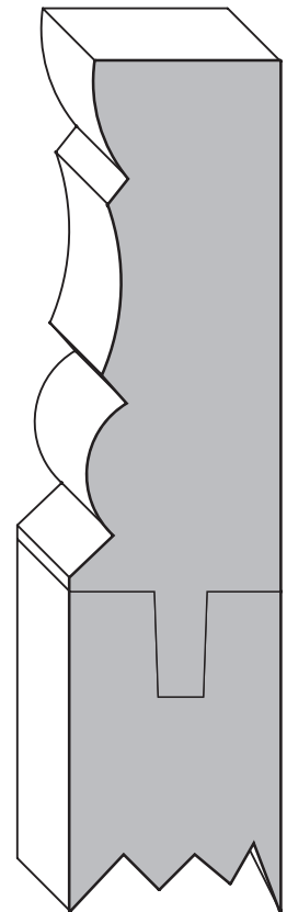
1015 1" x 2 7/16" (Top) Add 1/2" for tongue Bottom can be made up to 9" wide
