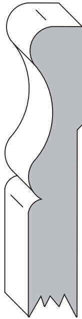
1029 9/16" thick up to 4 1/2" wide
