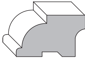
3059 3/4" x 1 1/4" (No size alterations)
