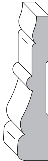
2024 w/ E1E 1/8" 9/16" x (2 1/2" max.)
