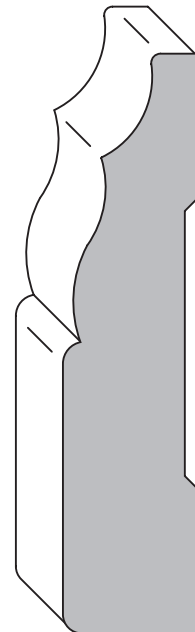
2029 w/ E1E 1/8" 11/16" x (5" max.)
