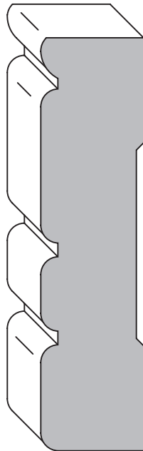
2015 w/ E1E 1/8" 3/4" x (3" max.)
