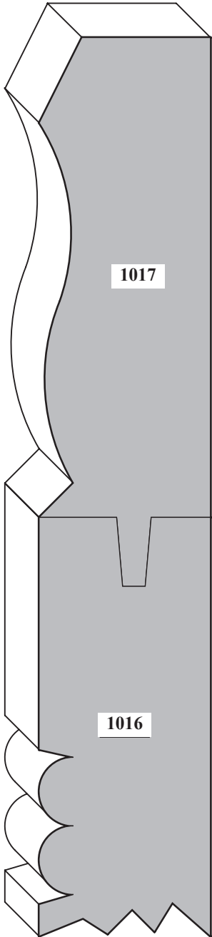
1016/1017 1 1/4" x 3 1/2" (top) Add 1/2" for tongue Bottom can be made up to 6 1/2" wide
