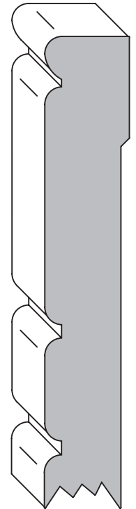
1024 5/8" thick up to 5 1/2" wide
