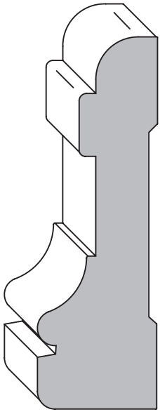
2001 w/ E1E 1/8" 7/8" x (2 3/4" max.)
