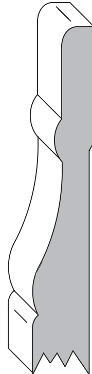
1020B 5/8" thick up to 5" wide
