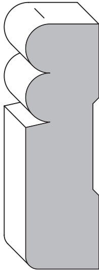
2041 w/ E1E 1/8" 3/4" x (2 1/2" max.)
