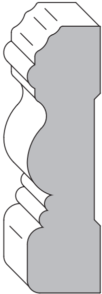
2018 w/ E1E 1/8" 3/4" x (2 3/4" max.)
