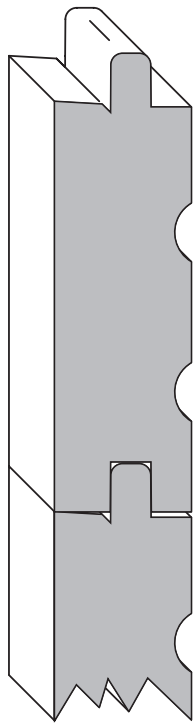
6001 3/4" x 2 1/4" (face) Flooring Up to 9" (face) Add 1/4" for tongue
